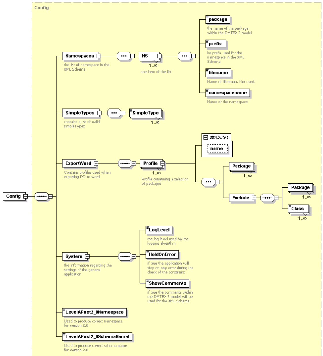
Figure 5 - XML Schema of the configuration file
